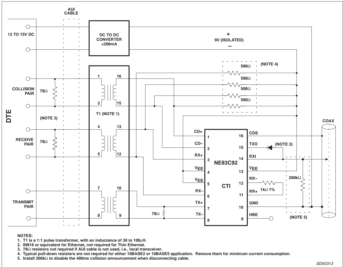
Figure 3. Connection Diagram for Standard 8392 Applications
