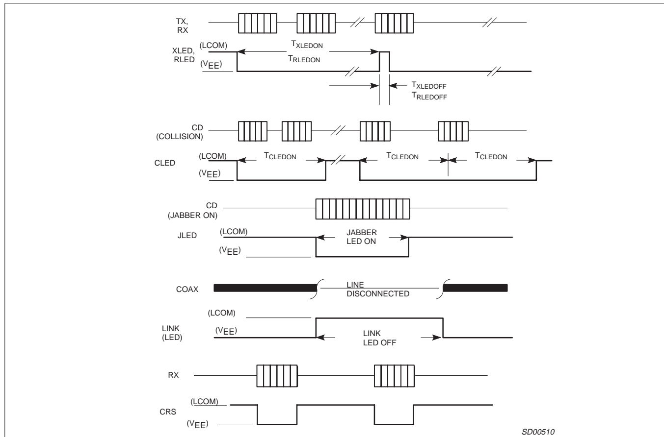
Figure 12. LED Timing
