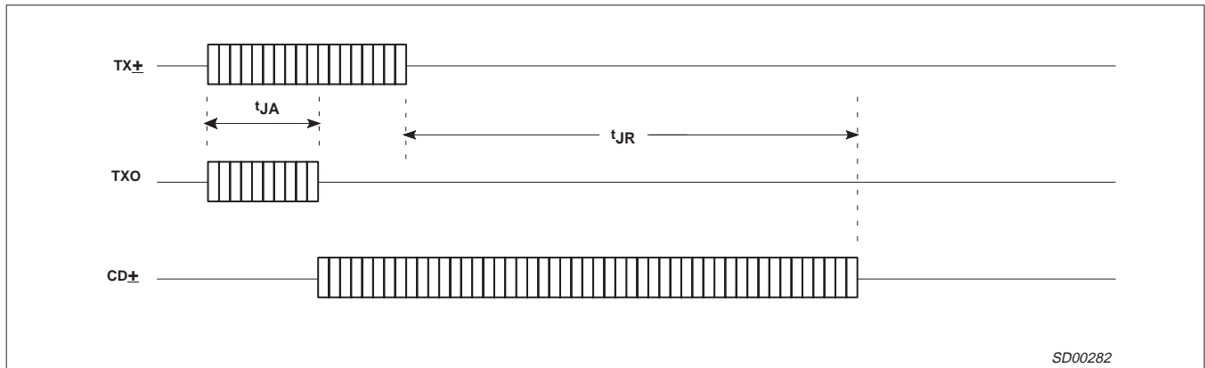
Figure 11. Jabber Timing
