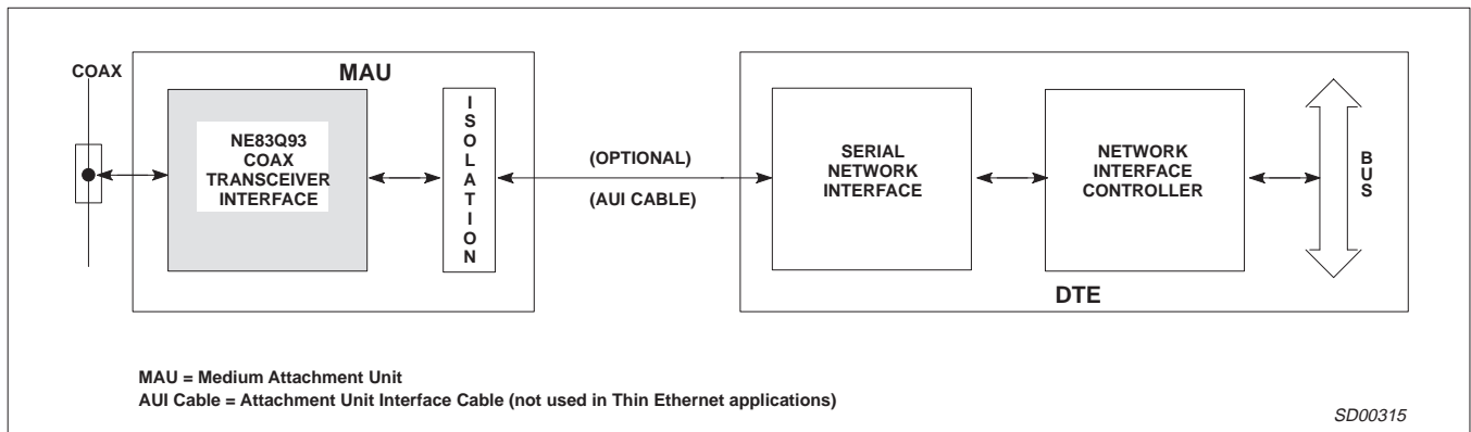
Figure 5. Interface Diagram for Ethernet/Thin Ethernet Local Area Network
