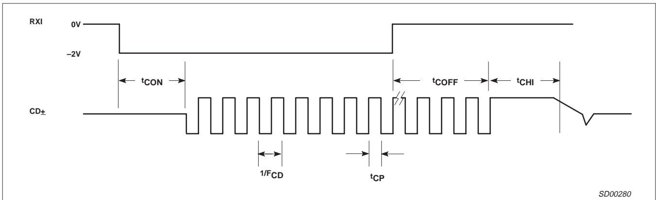
Figure 9. Collision Timing
