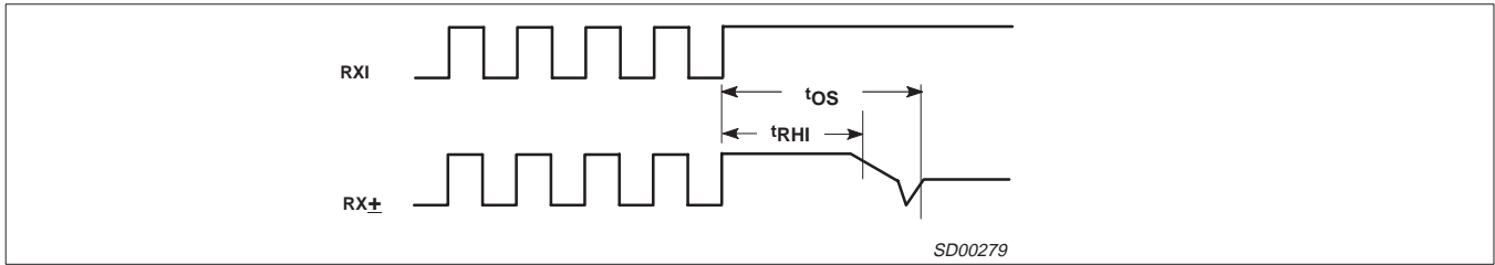
Figure 7. Receiver End-of-Packet Timing
