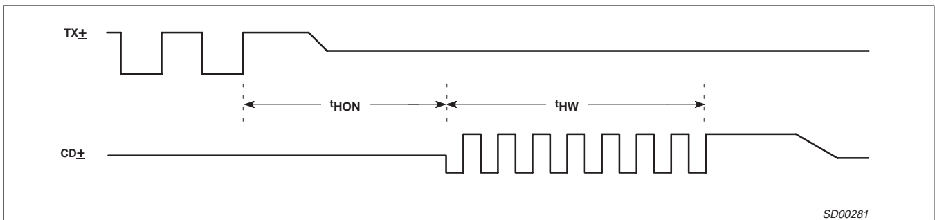
Figure 10. Heartbeat Timing
