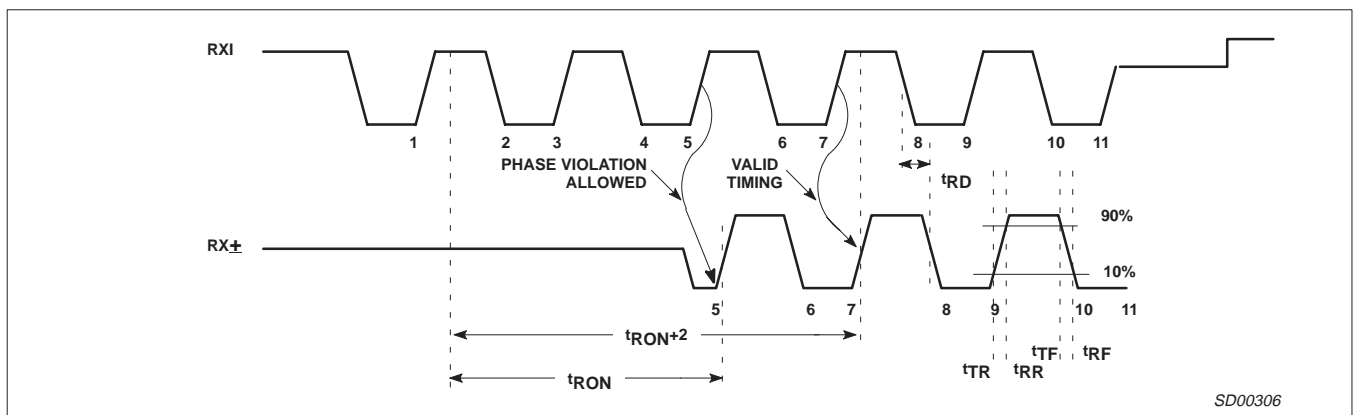
Figure 6. Receiver Timing
