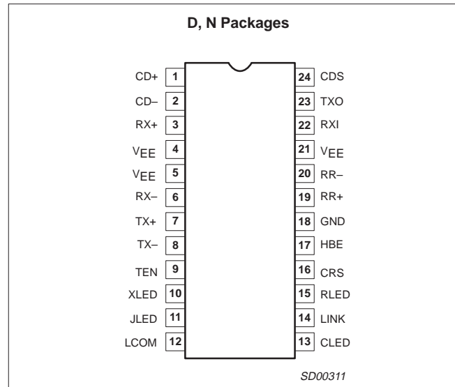
Figure 1. Pin Configurations
