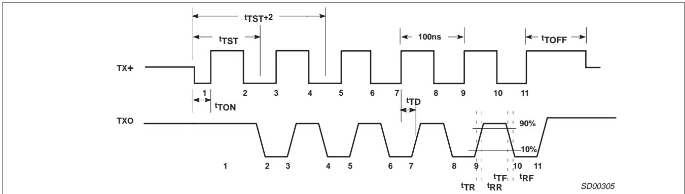
Figure 8. Transmitter Timing
